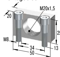
MB20SC2-V4A Montageblock
