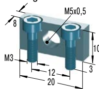
MB5SC2 Montageblock
