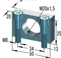
MB20SC2 Montageblock
